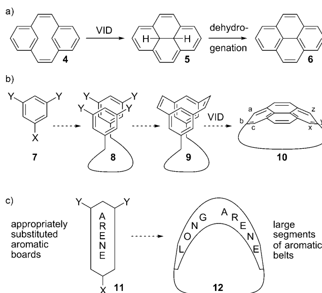
Scheme 1. The parent VID reaction of [2.2]metacyclophane-1,9-diene ( 4 ) to give pyrene ( 6 ), its use in the synthesis of [n](2,7) pyrenophanes ( 10 ) and a strategy for the synthesis of large [n] cyclophanes ( 12 ).
