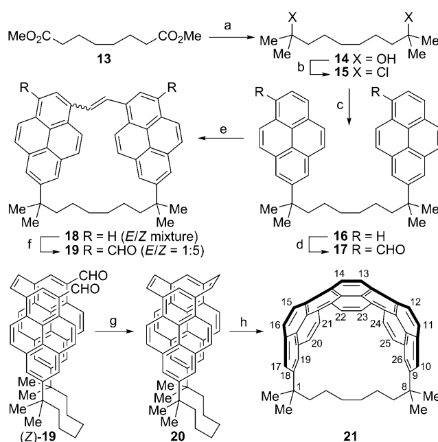
Scheme 2. Synthesis of 1,1,8,8-tetramethyl[8]-(2,11)teropyrenophane ( 21 ). Reagents and conditions: a) MeMgBr, THF, 0 °C to reflux, 10 h, 86%; b) 12 M HCl (aq), RT, 2 h, 91%; c) pyrene ( 6 ), AlCl 3 , CH 2 Cl 2 , 0 °C to RT, 4 h, 62%; d) Cl 2 CHOCH 3 , TiCl 4 , CH 2 Cl 2 , 0 °C to RT, 2 h, 88%; e) TiCl 4 , Zn, pyridine, THF, 0 °C to reflux, 5 h; f) Cl 2 CHOCH 3 , TiCl 4 , CH 2 Cl 2 , 0 °C to RT, 2 h, 11% ( E )- 19 , 57% ( Z )- 19 ; g) TiCl 4 , Zn, pyridine, THF, 0 °C to reflux, 4 h, 41%; h) DDQ, m -xylene, 145 °C, 48 h, 95%. DDQ = 2,3-dichloro-5,6-dicyano-1,4-benzoquinone.
