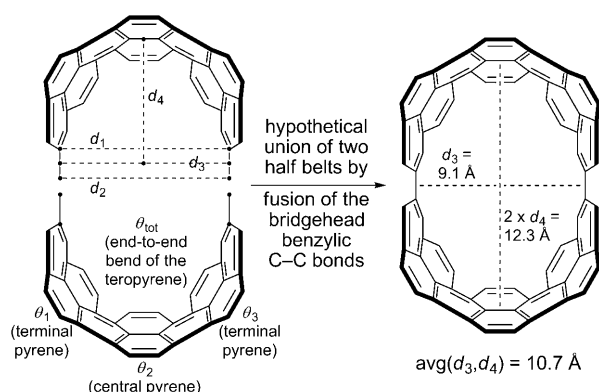
Figure 3. Parameters used to describe the structure of 21 and the hypothetical joining of two half belts to afford an ellipsoidal segment of an (8,8) armchair SWCNT.
